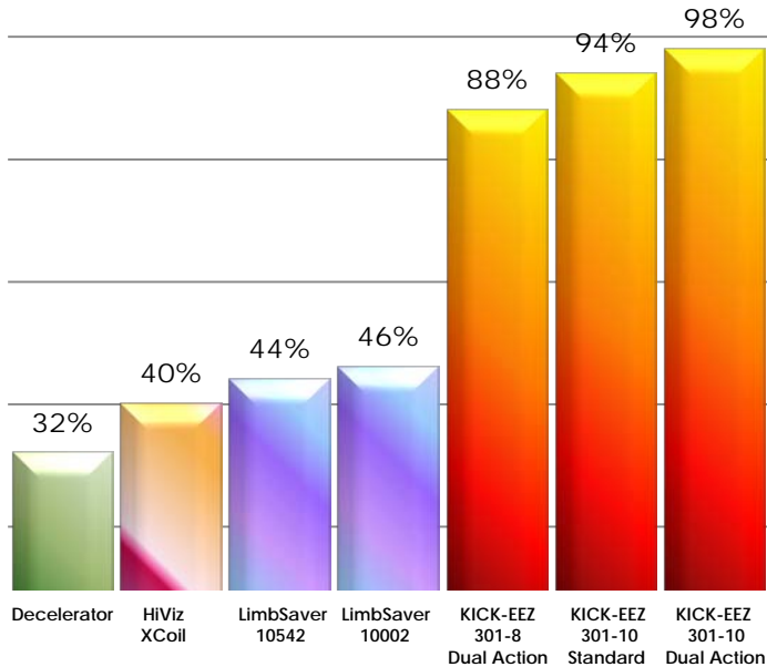
Energy Absorbed by Recoil Pads
